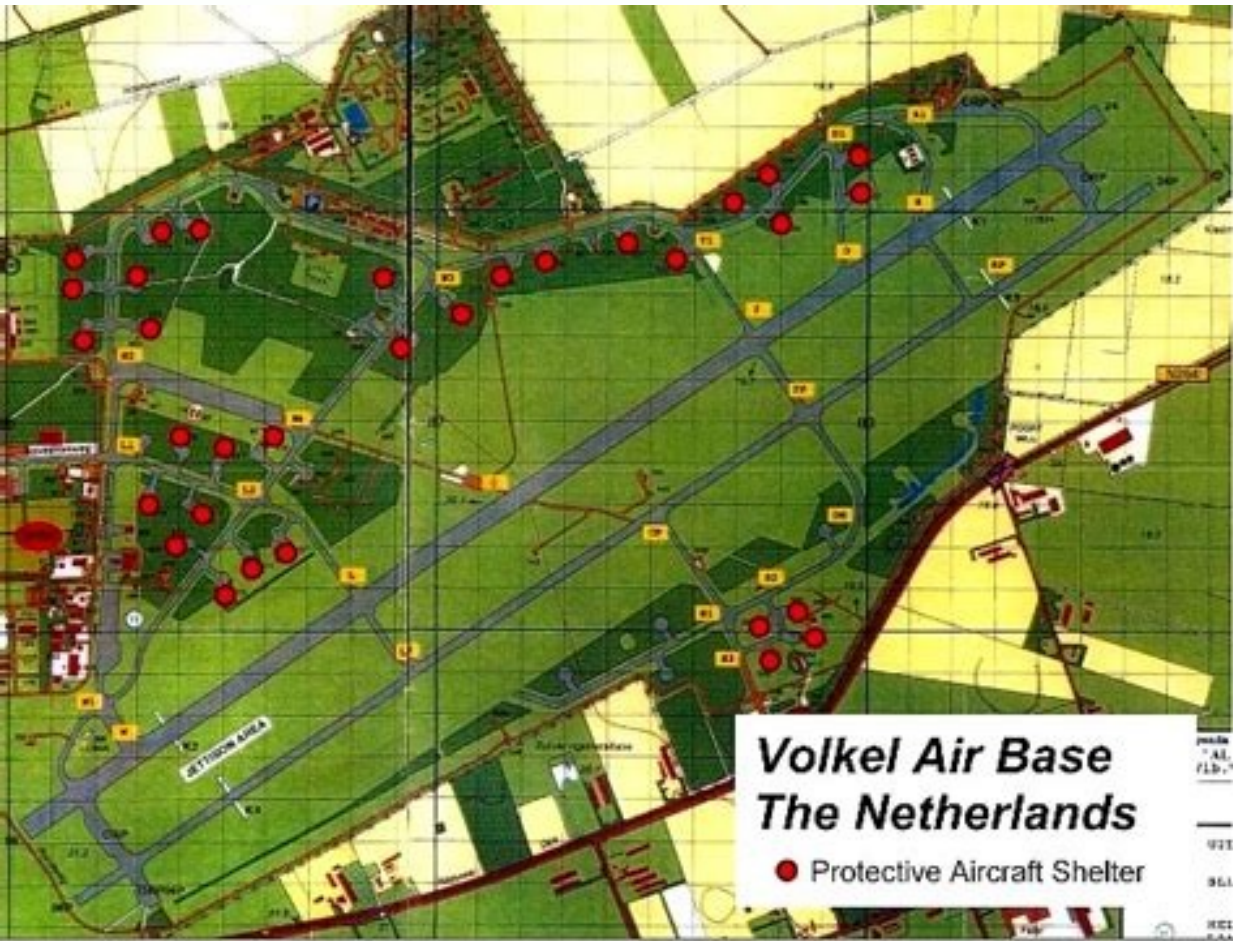
Volkel Air Base, the Netherlands (July 20, 1999): The base is located in the southeastern parts of the Netherlands (51°39'N, 05°43' E). There are 32 Protective Air Shelters (PAS) on the base, 11 of which are equipped with WS3 Weapons Storage Vaults for nuclear weapons storage with a capacity of 44. The vaults were completed in 1991. Twenty B61 bombs are stored at the base for delivery by Dutch F-16A/Bs of the 311 th and 312 th fighter squadrons.
